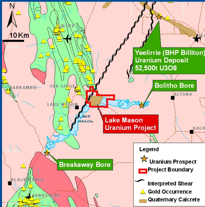
Similar source rocks to Yeelirrie
